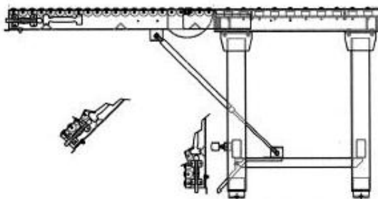
BTU-04 Similar to ROL-42 - Ball Deck Table with Gravity Roller Drop Gate
